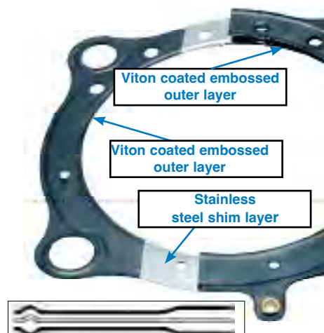
3 Layer MLS Style Cross Section
